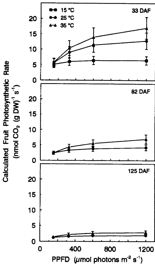
Fig. 5. Fruit photosynthetic rates per unit dry weight of late-maturing cv. Cal Red peaches, calculated from data in Fig. 4, in response to light at 15 (early in the season), 25 and 35°C and at 33, 82 and 125 DAF (mean \pm SE of 3-4 measurements; SE bars are visible when larger than the symbols depicting data points).
