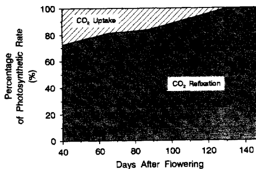
Fig. 8. CO 2 uptake and CO 2 refixation as a percentage of calculated fruit photosynthetic rates during the growing season calculated from data in Fig. 7.
