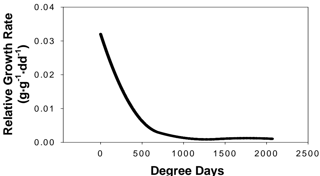
Fig. 1. The general relative growth rate pattern for a late maturing peach cultivar. Time is expressed in day degrees to account for the influence of temperature on developmental rate. Source: Grossman and DeJong, 1995a.
