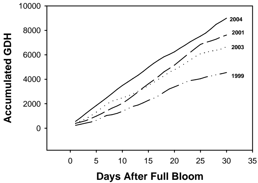
Fig. 3. A comparison of heat accumulation (growing degree hours) during the first thirty days after bloom for 2004 compared to three previous years. Data from the Parlier weather station in Fresno County as accessed through fruitsandnuts.ucdavis.edu .
