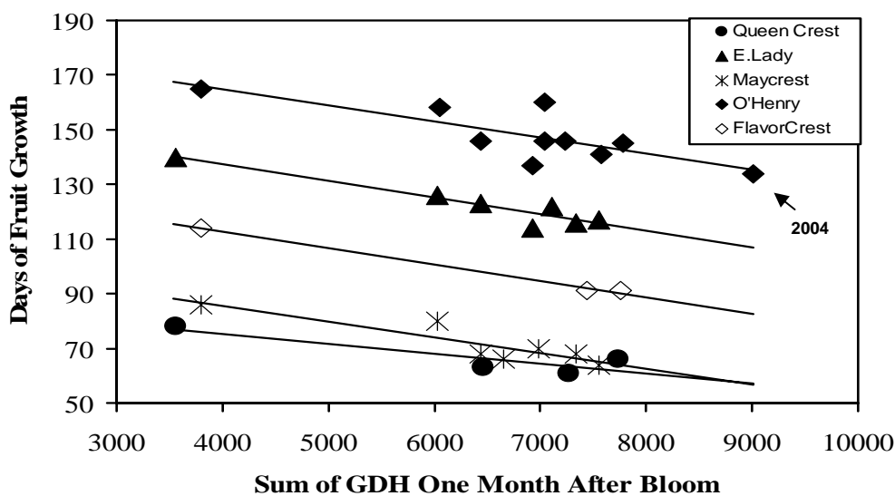
Fig. 2. The relationships between days of fruit growth (bloom to harvest) and the accumulation of heat (growing degree hours) over the first 30 days after bloom for five different peach cultivars. The 2004 point on the O'Henry line indicates how well the previous model fits the 2004 data. Source: Ben Mimoun and DeJong, 1999.
